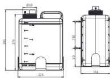
• 07220096 Below Deck Multifeed Kit
