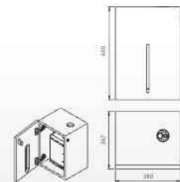
• 07220096CB Below Deck Multifeed Kit With lockable cabinet
