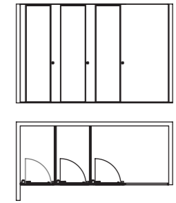
OPTION 3: INLINE TOILET CUBICLE
