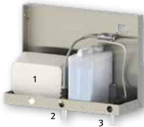
Modular system including high-speed hand dryer (1), touch-free faucet (2) and liquid soap dispenser (3)
